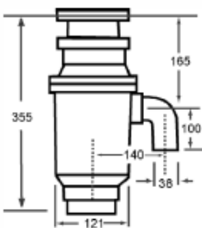
Builder, Standard
